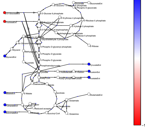
(c) Chemical potentials (kJ/mol)
