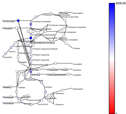
(g) Reaction elasticities
