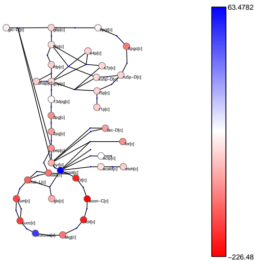
(c) Chemical potentials (kJ/mol)
