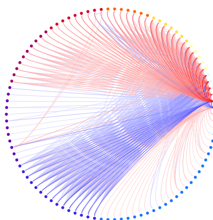
Figure 3: Synergies: statistics
