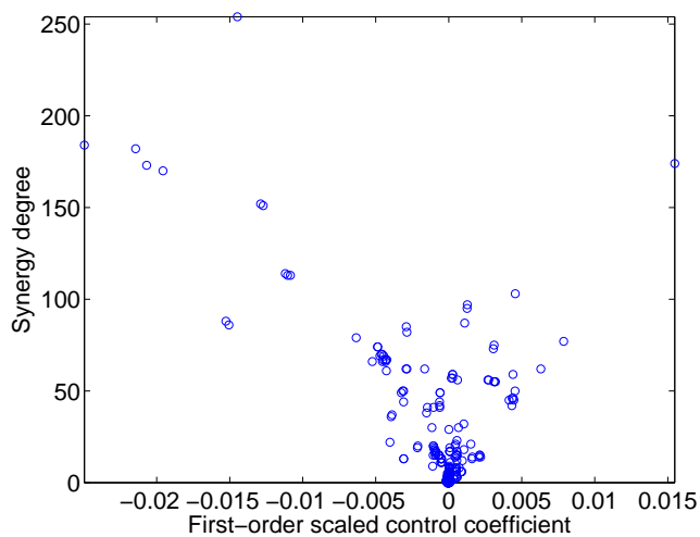
Synergy degrees and scaled control
