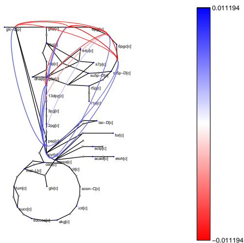
Synergy degree distribution
