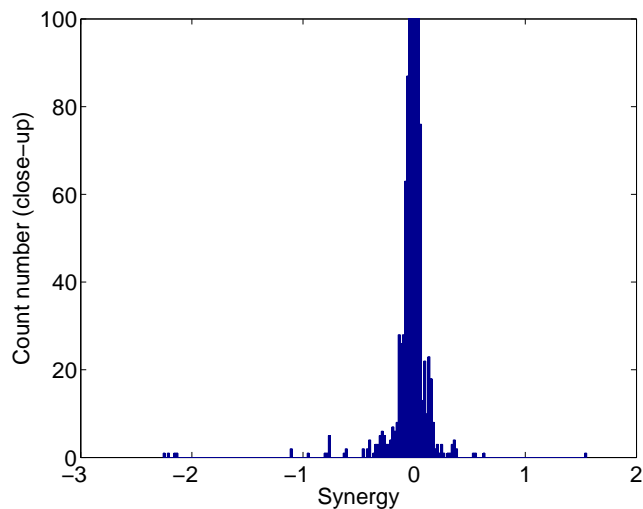
Synergies
