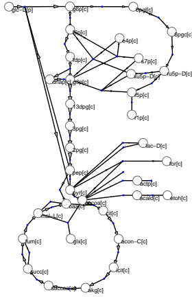
(c) Chemical potentials (kJ/mol)
