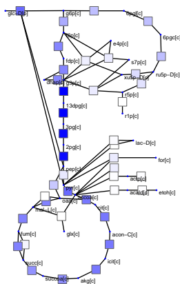
(g) Reaction elasticities
