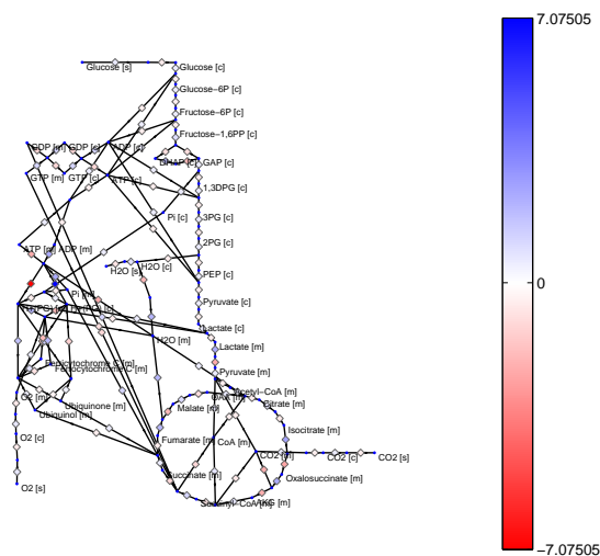
Figure 2: Model construction step by step (continued). (e) Local dissipation of Gibbs free energy (driving force multiplied by flux). (f) Saturation values. (g) Scaled elasticities. (h) Scaled enzyme response coefficients, predicted by elasticity sampling. Positive values are shown in blue, negative values in red, zero values in white.
