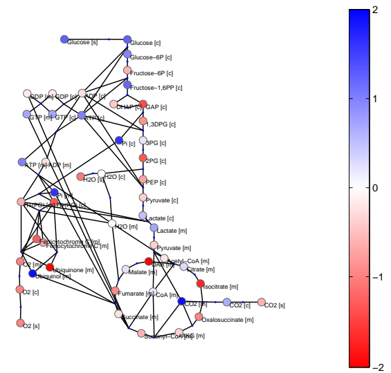
(b) Concentrations (mM)
