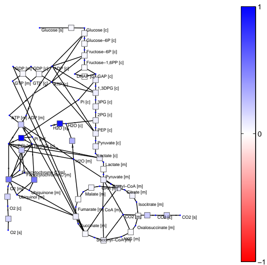
(h) Flux response
