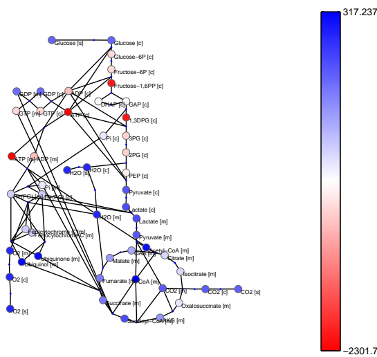
(c) Chemical potentials (kJ/mol)
