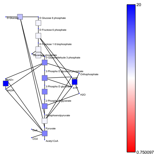
(g) Reaction elasticities
