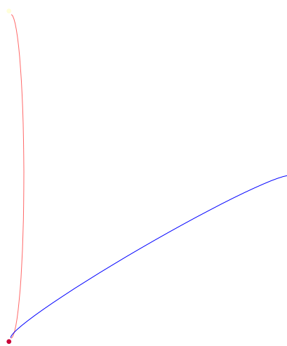
Figure 3: Synergies: statistics
