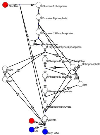
(a) Metabolic fluxes (mM/s)
