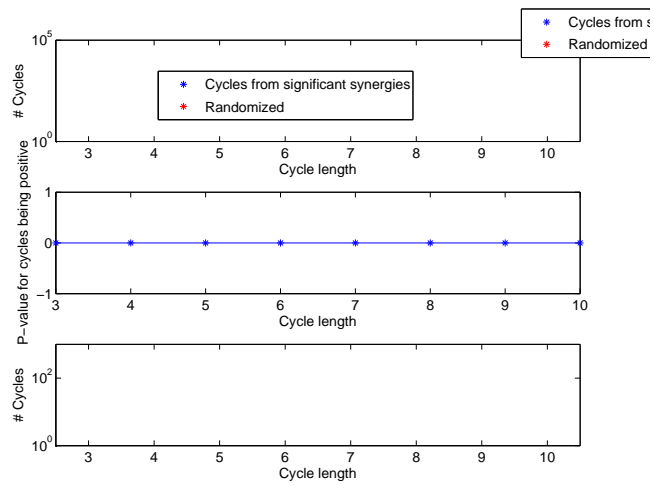
Figure 5: Statistics of synergy cycles
