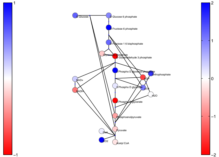
(b) Concentrations (mM)
