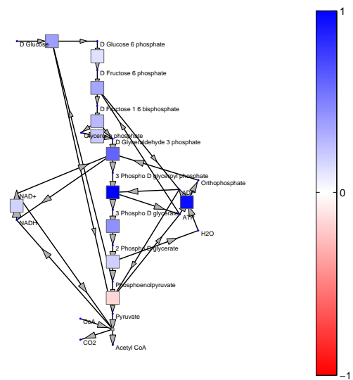
Figure 2: Model construction step by step (continued). (e) Local dissipation of Gibbs free energy (driving force multiplied by flux). (f) Saturation values. (g) Scaled elasticities. (h) Scaled enzyme response coefficients, predicted by elasticity sampling. Positive values are shown in blue, negative values in red, zero values in white.
