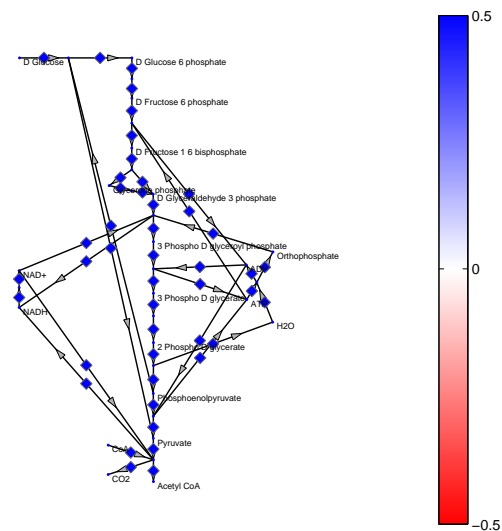
(f) Enzyme saturation
