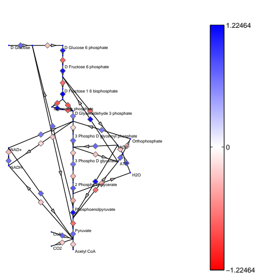
(g) Reaction elasticities
