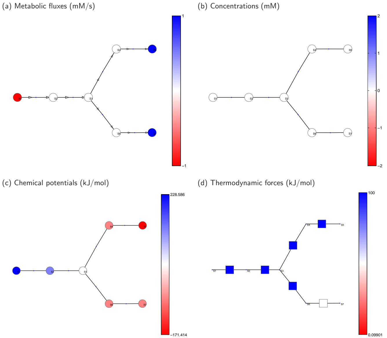
Figure 1: Model construction step by step. (a) Thermodynamically feasible flux distribution (grey arrows). (b) Metabolite levels. (c) Chemical potentials. (d) Thermodynamic driving forces.
