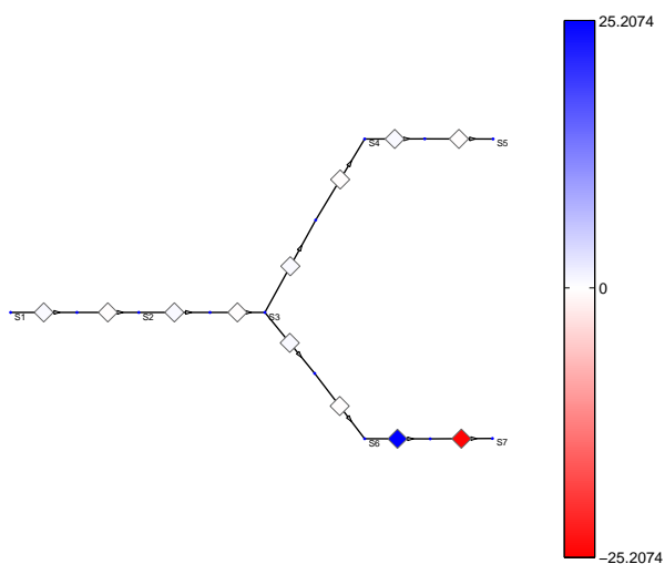
Figure 2: Model construction step by step (continued). (e) Local dissipation of Gibbs free energy (driving force multiplied by flux). (f) Saturation values. (g) Scaled elasticities. (h) Scaled enzyme response coefficients, predicted by elasticity sampling. Positive values are shown in blue, negative values in red, zero values in white.
