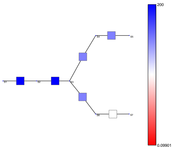
(g) Reaction elasticities
