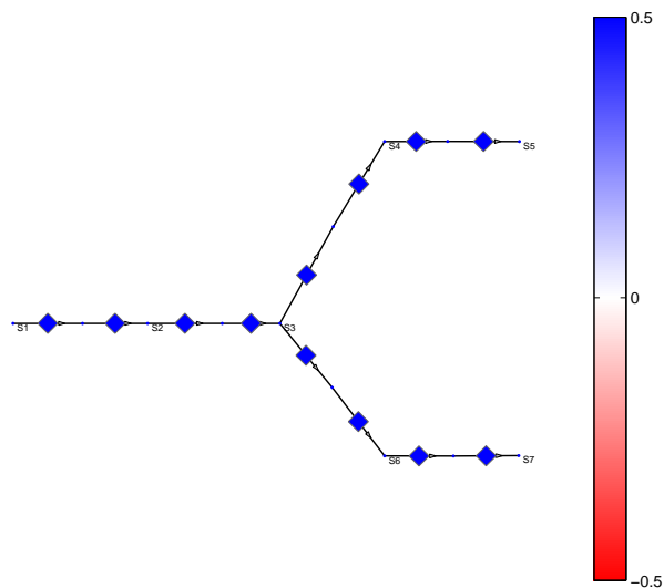
(f) Enzyme saturation
